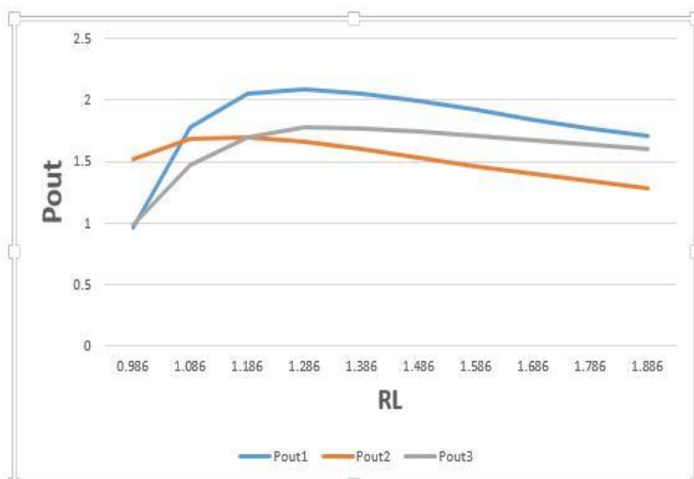
Figure 5. Effects of load variation on output power ( P_{out} )
