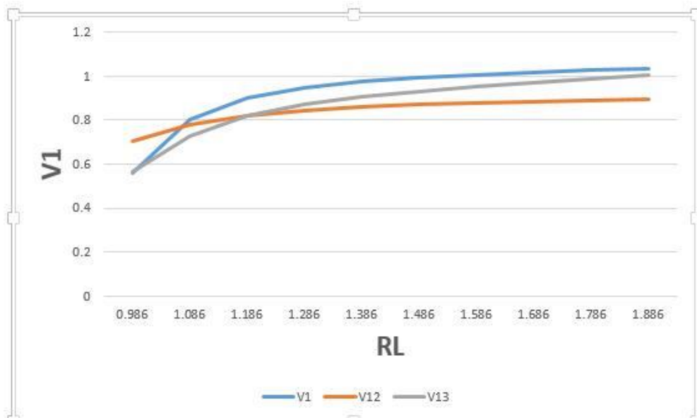
Figure 4. Effects of load variation on load voltage (V1)
