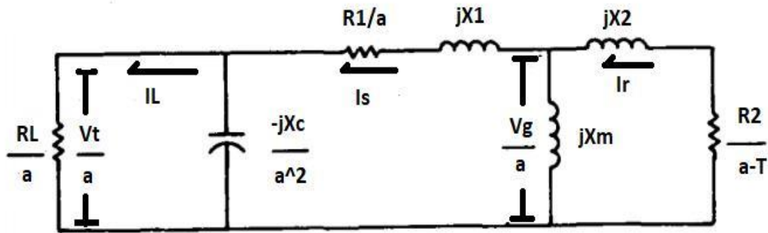
Figure 1. Equivalent circuit of the induction generator with load
