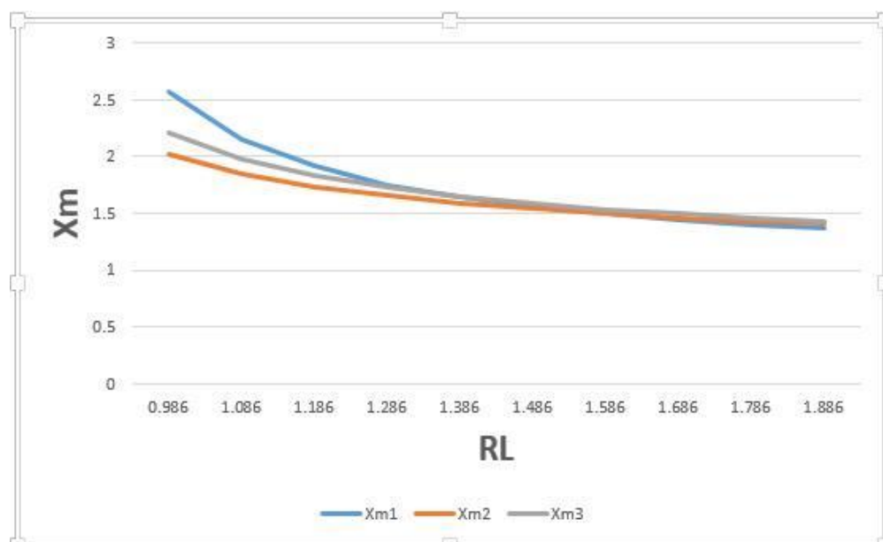
Figure 2. Effects of load variation on magnetizing reactance ( X_m )
