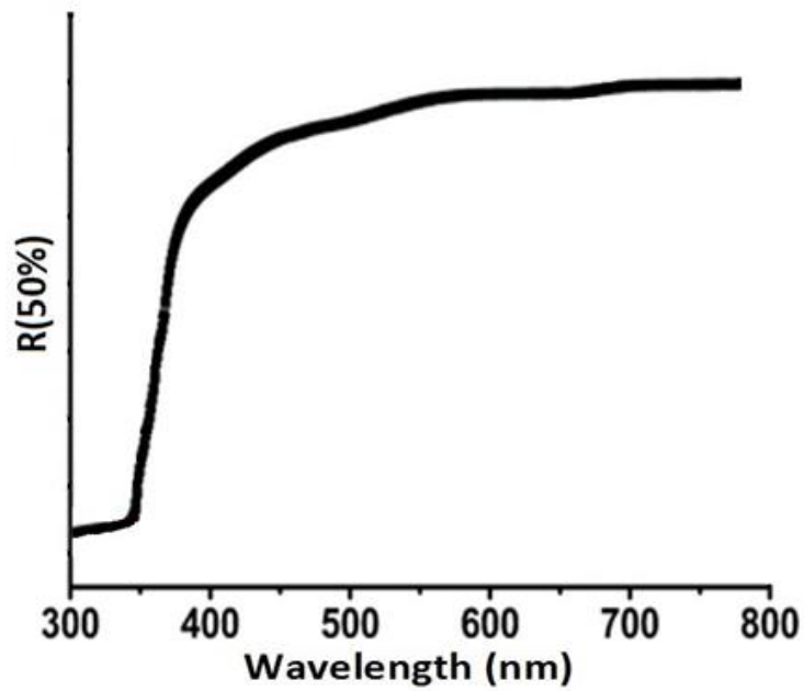
Figure 3. Diffuse reflectance spectra of ZnO thin film.
