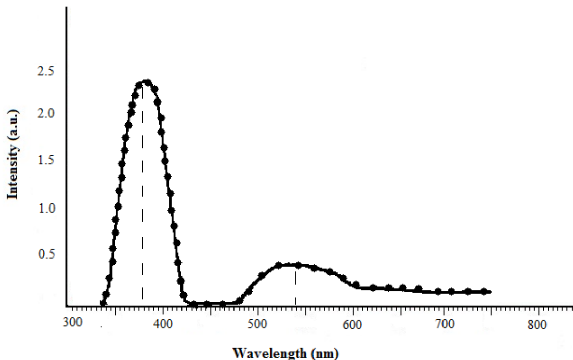
Figure 5. Photoluminescence spectrum of ZnO thin film.
