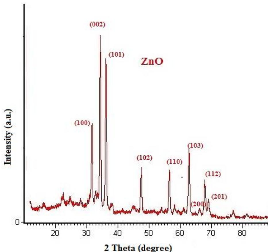
Figure 1. X-Ray diffraction (XRD) spectra of ZnO thin film.
