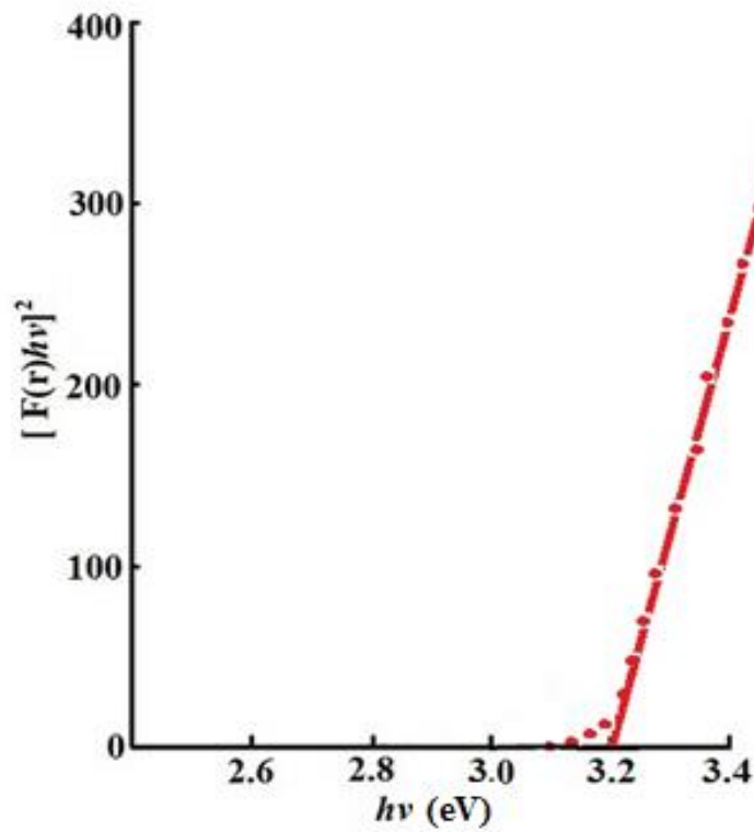
Figure 4. Plot of [F(R) hv]^2 versus photon energy ( h\nu ) for ZnO thin film
