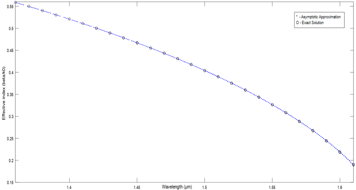
Fig. 2. Propagation Constants
