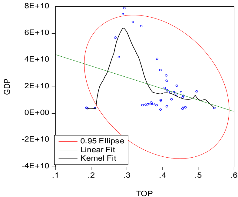
Figure 1. The confidential ellipse between the variables Source: E-view software
