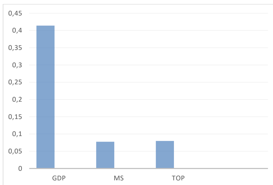
Figure 2. Volatility of the variables
