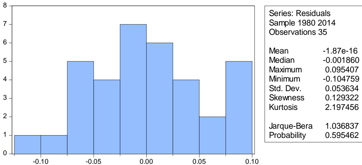
Figure 3. The residual normality test
