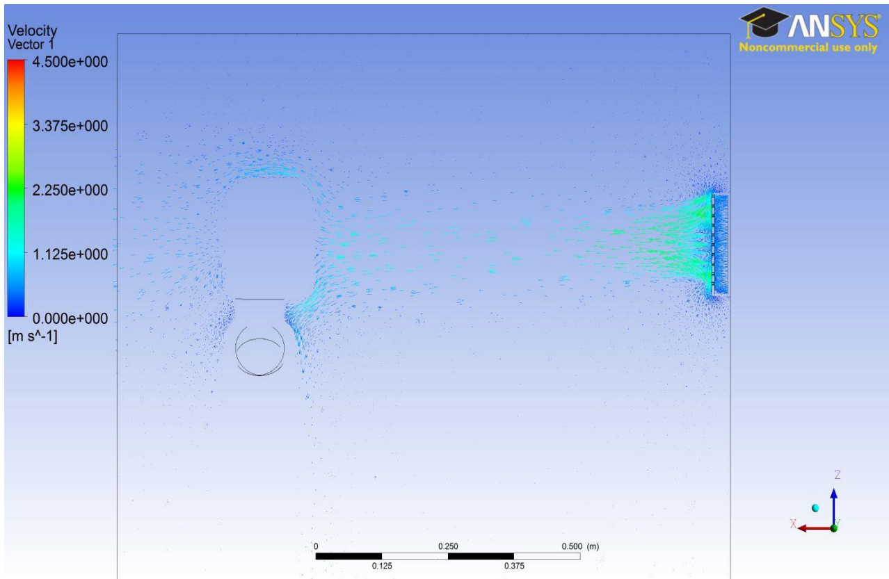
Figure 3. Medium flow rate through the personal ventilation system.
