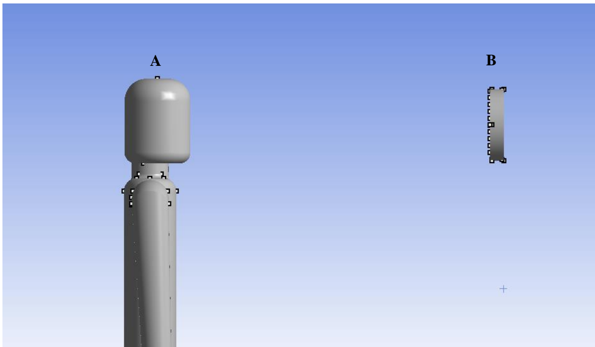
Figure 1. Layout of the test objects in the Ansys modeler. A: view of the upper body of the sitting occupant, B: air terminal device (air inlet)
