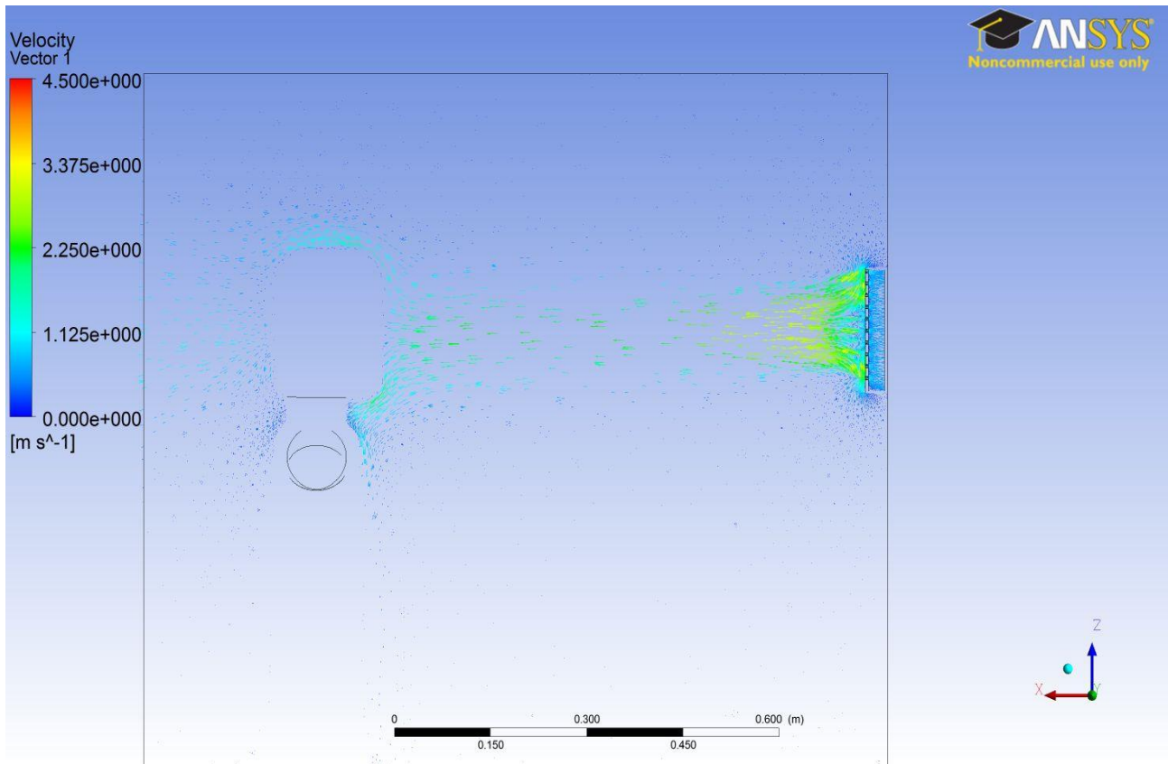
Figure 2. Maximum flow rate through the personal ventilation system.
