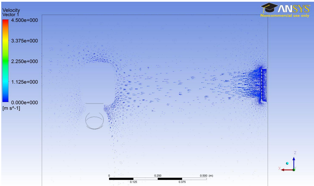
Figure 5. flow rate through the personal ventilation system equal to 1L/s.
