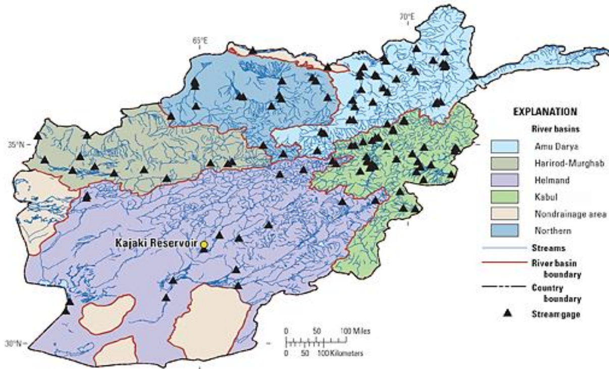
Figure 2. Locations of Afghanistan’s major drainage basins, reinstalled streamgauge stations and the Kajaki Reservoir, a major source for hydropower and irrigation in the Helmand River Basin. Credit: Thomas J. Mack, USGS. [8].
