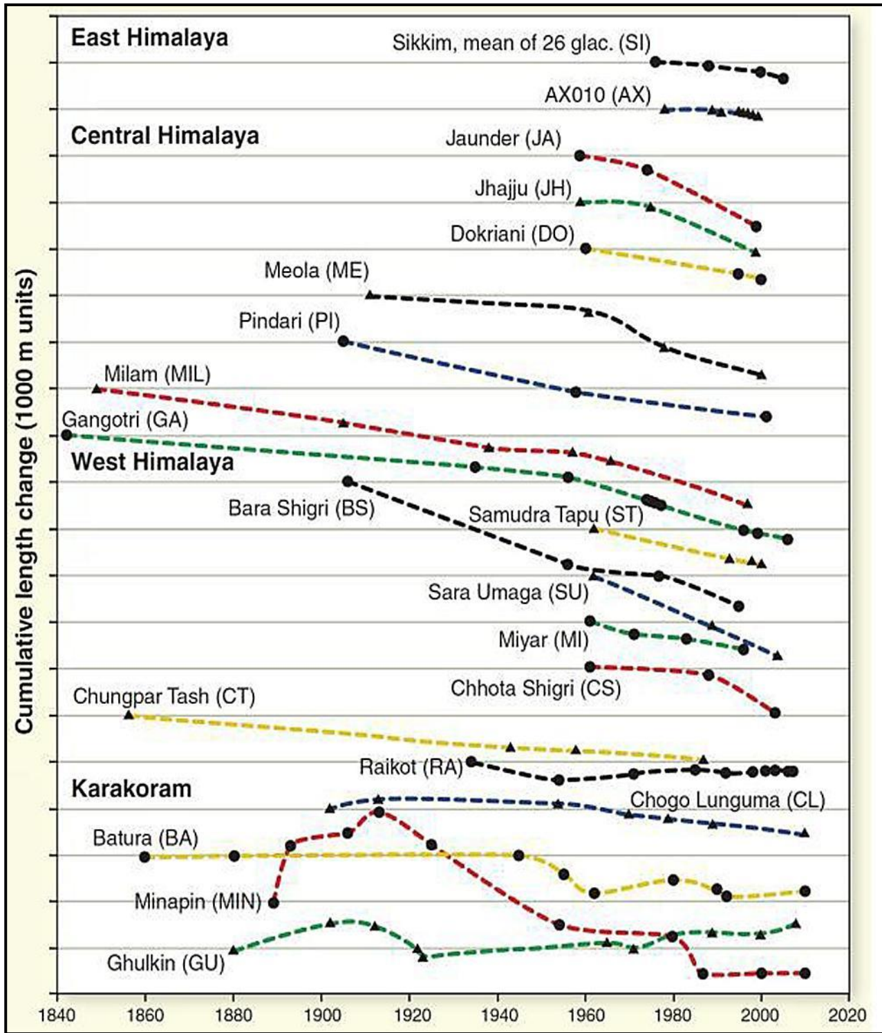
Figure 1. Most of the Himalayan glaciers show retreat since the mid-19th century, except the glaciers at Nanga Parbat in the northwest (RA, CL) and glaciers in the Karakoram, which show a complex behaviour (Bolch et al., 2012).
